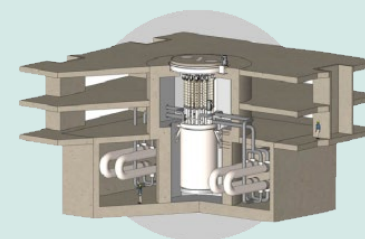
KP-FHR Fluoride salt-cooled high-temperature reactor KAIROIS POWER
