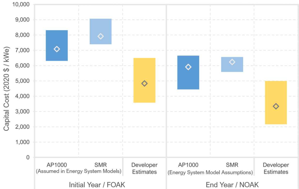
Figure 1. Default Capital Costs Used in Energy System Models and Capital Costs Reported by Advanced Nuclear Reactor Developers
